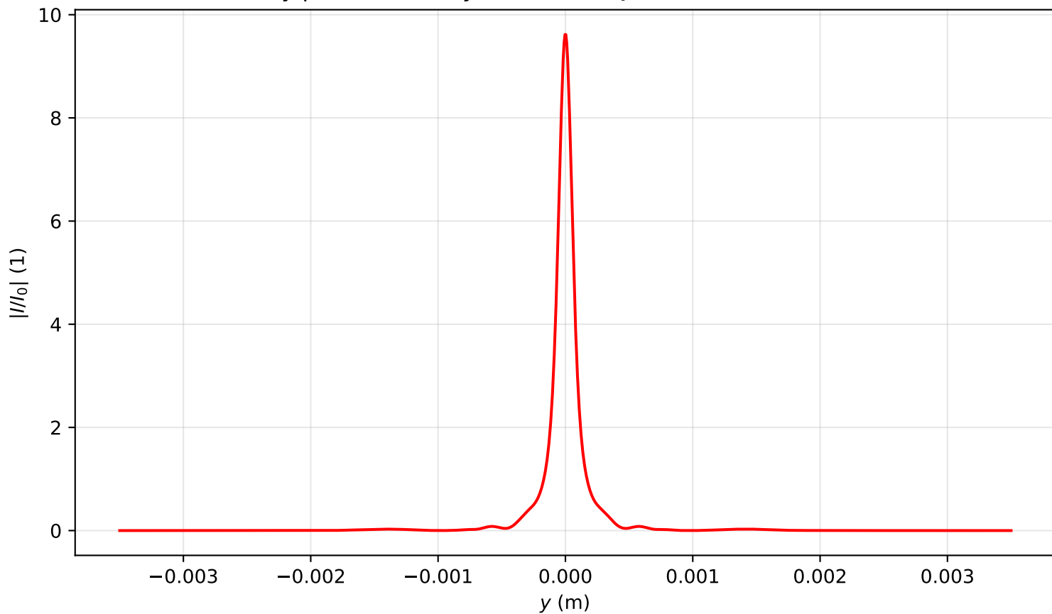
Intensity profile I(x=0, y, z=2.149)/I_0 , \text{Pin}=2.5\text{Pcr} , artificial time
